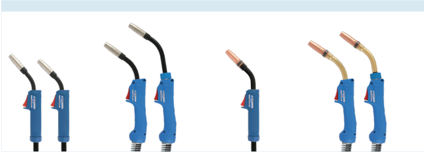
TBi 140/145 60% (10 min.) Mix: 140 A CO 2 : 160 A Ø 0.6-1.0 mm
